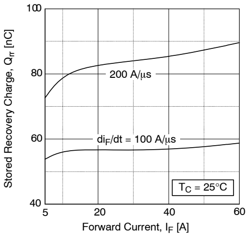
Figure 21. Stored Charge
