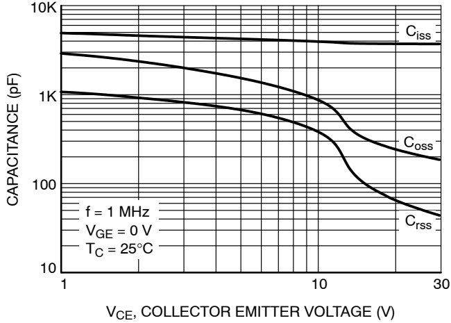
Figure 7. Capacitance Characteristics
