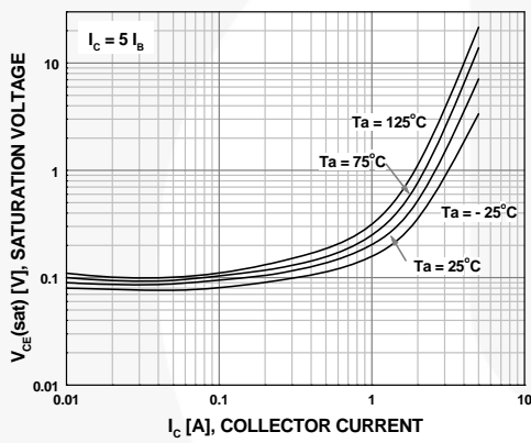
Figure 3. Saturation Voltage
