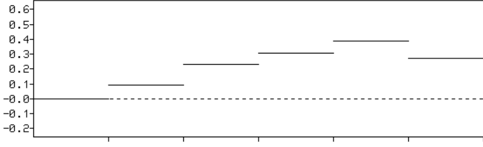
Figure 7. Differential Gain
