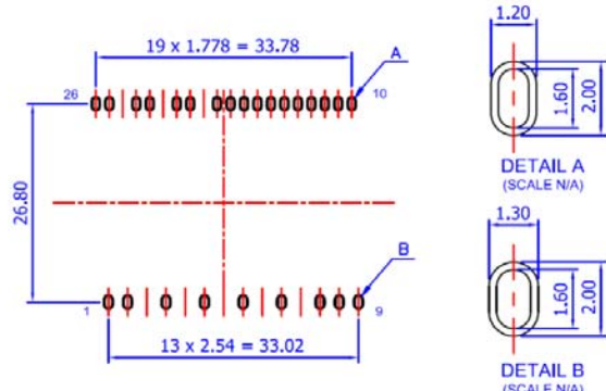
LAND PATTERN RECOMMENDATIONS
