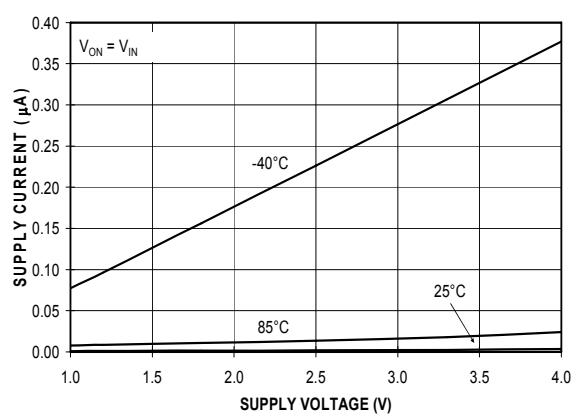
Figure 13. Quiescent Current vs. Supply Voltage (V ON =V IN )
