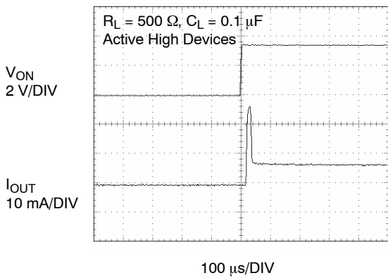
Figure 20. T ON Response
