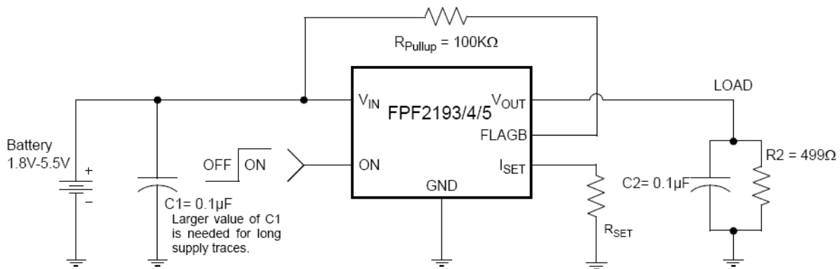
Figure 28. Typical Application
