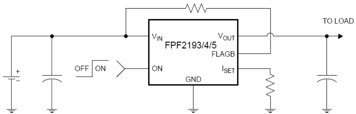
Figure 1. Typical Application
