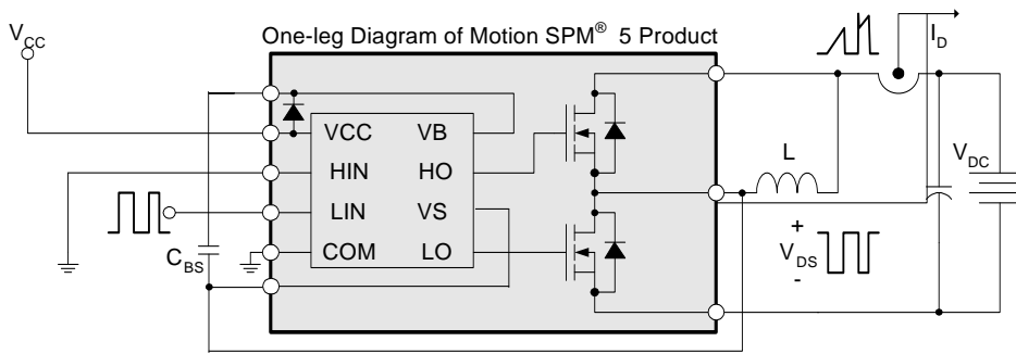
Figure 6. Switching and RBSOA (Single-pulse) Test Circuit (Low-side)
