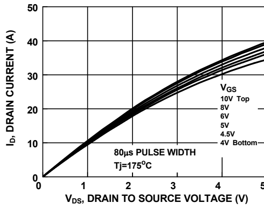
Figure 10. Saturation Characteristics
