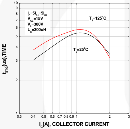
Figure 15. Inductive Switching Time, t_{strG}
