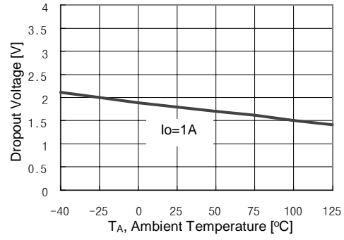
Figure 4. Dropout Voltage
