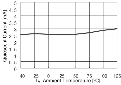
Figure 3. Quiescent Current
