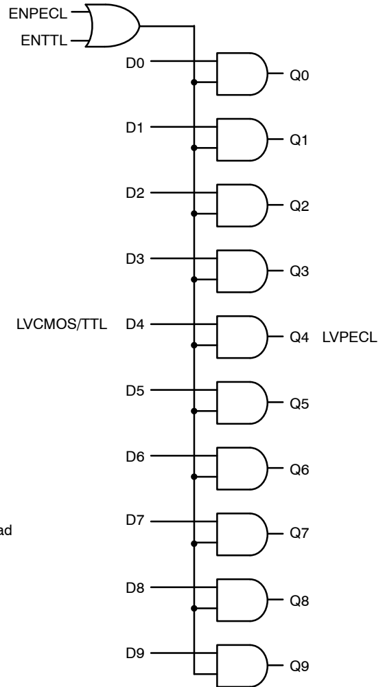
Figure 2. Logic Symbol
