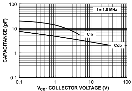
Figure 6. Input and Output Capacitance vs Reverse Voltag
