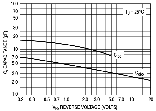
Figure 8. Capacitances
