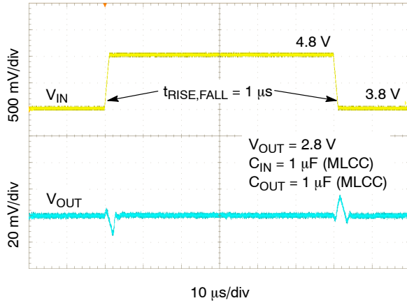
Figure 34. Line Transient Response – IOUT = 10 mA
