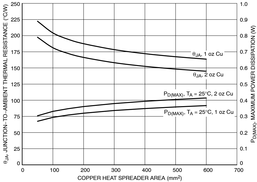
Figure 46. θ JA and P D(MAX) vs. Copper Area (TSOP-5)
