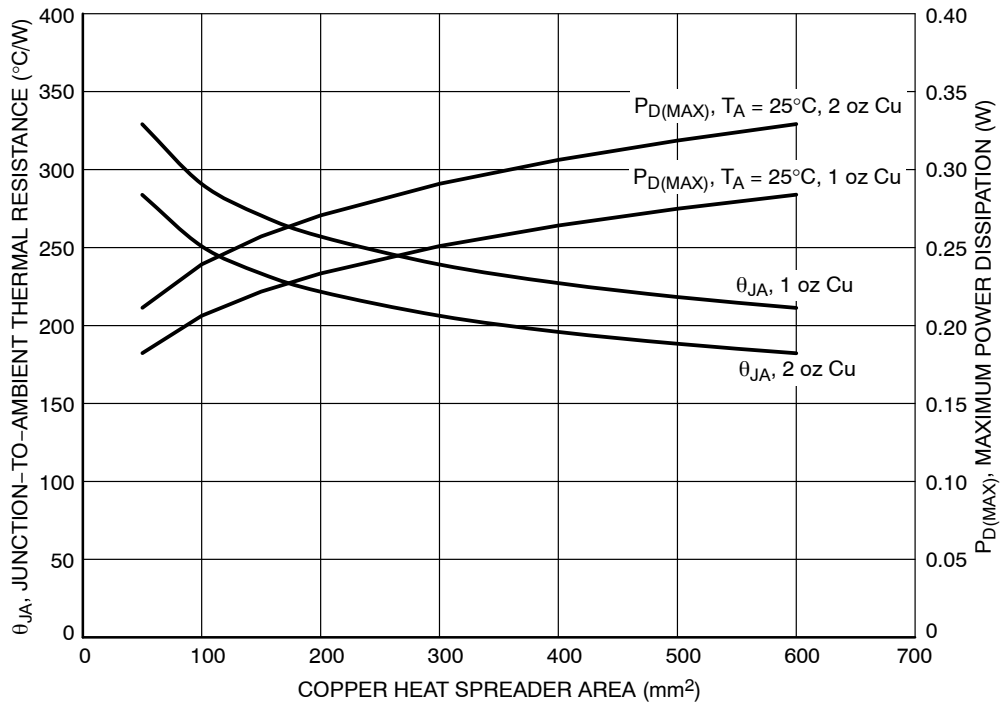
Figure 45. θ JA and P D(MAX) vs. Copper Area (XDFN4)
