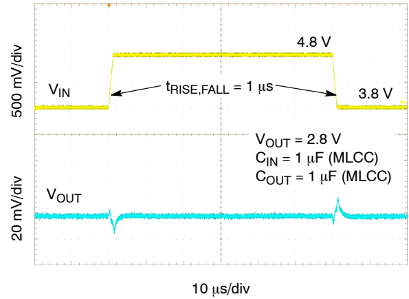
Figure 35. Line Transient Response – IOUT = 150 mA
