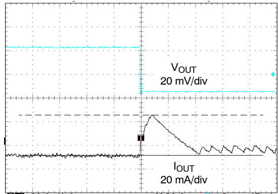
Figure 24. 100 mA to 10 mA Load Transient (V IN = 3.6 V, V OUT = 1.2 V, T A = 25°C)
