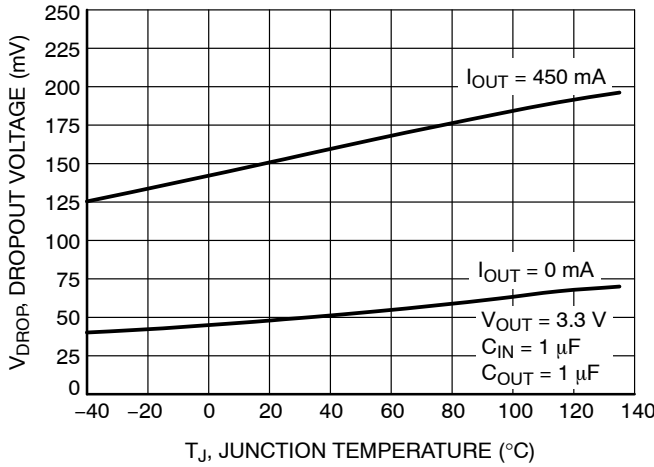
Figure 22. Dropout Voltage vs. Temperature– V OUT = 3.3 V
