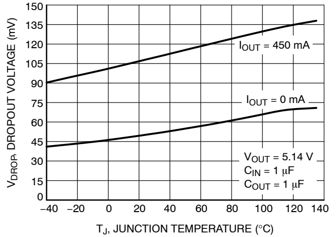
Figure 23. Dropout Voltage vs. Temperature– V OUT = 5.14 V
