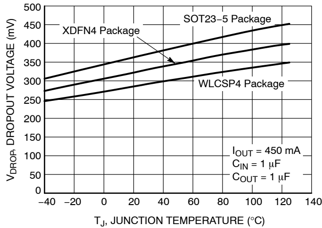
Figure 24. Dropout Voltage vs. Temperature V OUT = 1.8 V
