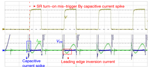
Figure 52. Leading Edge Inversion Current
