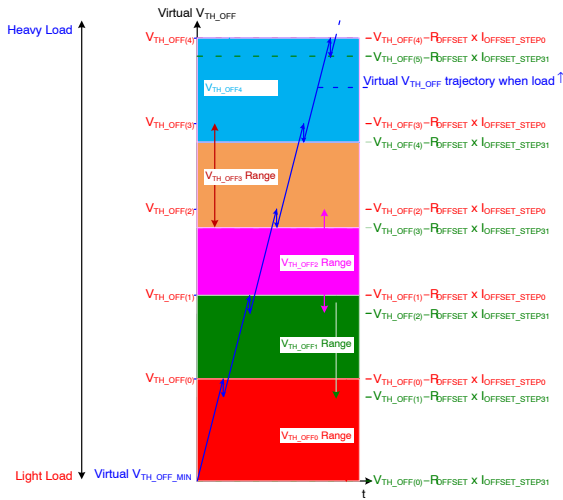
Figure 54. Virtual V_{TH\_OFF} Trajectory when lout Increases
