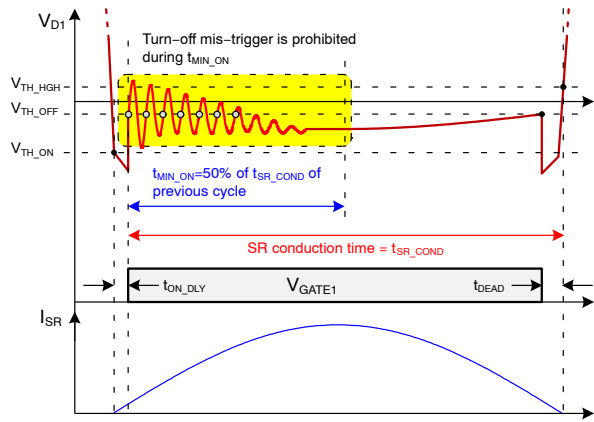
Figure 49. Minimum Turn-on Time and Turn-off Mis-triggering
