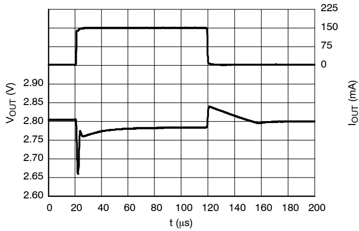
Figure 28. Load Transients, 2.8 V Version, I_{OUT} = 1 - 150 \text{ mA} , t_R = t_F = 0.5 \mu s , V_{IN} = 2.2 \text{ V} , AE = 0 \text{ V}
