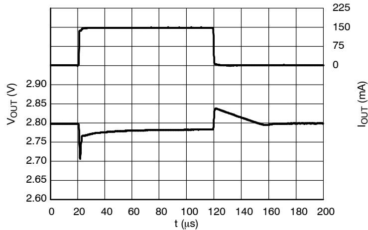
Figure 30. Load Transients, 2.8 V Version, I_{OUT} = 1 - 150 \text{ mA} , t_R = t_F = 0.5 \mu s , V_{IN} = 2.8 \text{ V} , AE = V_{IN} \text{ V}
