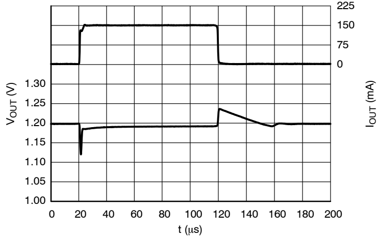
Figure 29. Load Transients, 1.2 V Version, I_{OUT} = 1 - 150 \text{ mA} , t_R = t_F = 0.5 \mu s , V_{IN} = 2.2 \text{ V} , AE = V_{IN} \text{ V}
