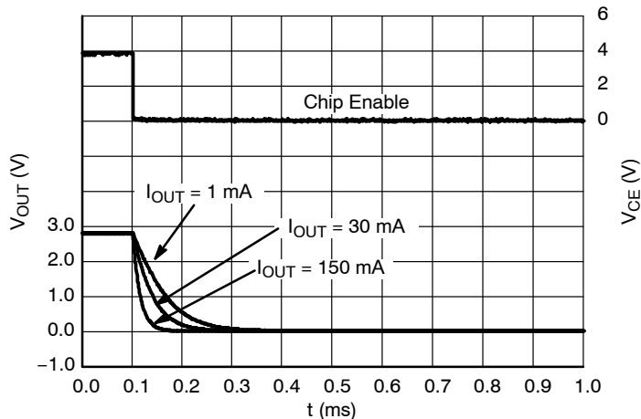
Figure 42. Shutdown, 2.8 V Version, V_{IN} = 3.8\text{ V}
