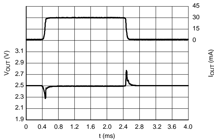
Load Transients, 2.5 V Version, I_{OUT} = 1 - 30 \text{ mA} , t_R = t_F = 50 \mu s , V_{IN} = 4.5 \text{ V}
