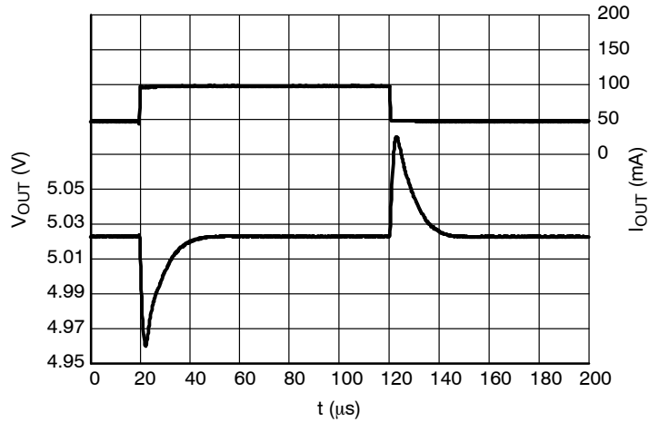
Figure 28. Load Transients, 8.0 V Version, I_{OUT} = 1 - 20 mA, t_R = t_F = 50 \mu s, V_{IN} = 11.0 V
