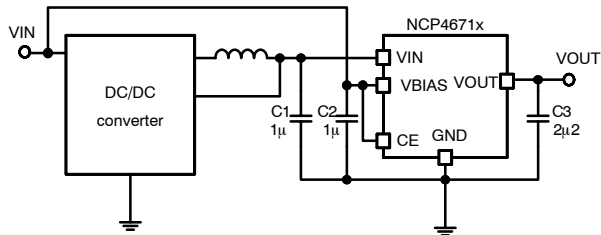
Figure 64. Typical Application Schematic with DC/DC Converter
