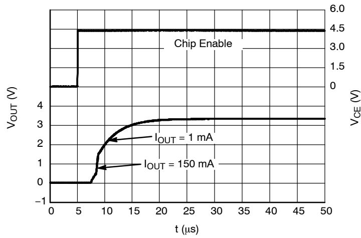
Figure 50. Start-up, 3.3 V Version, V_{IN} = 4.3 V
