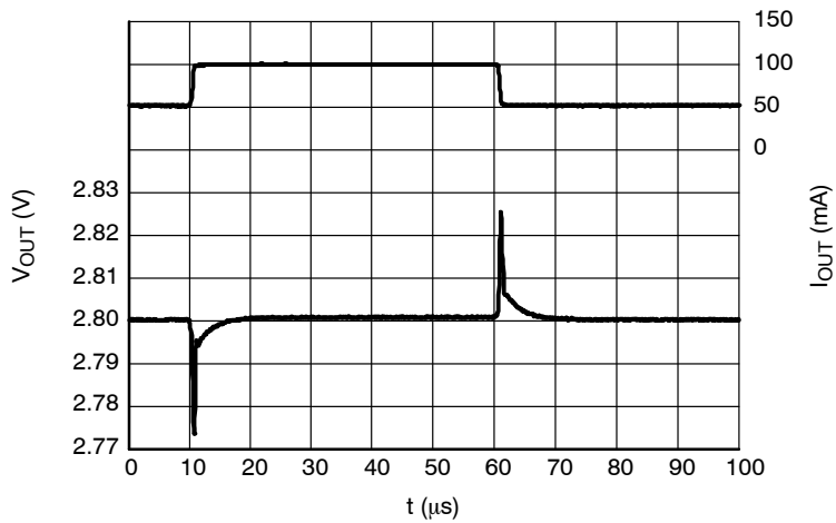
Figure 42. Load Transients, 3.3 V Version, I_{OUT} = 50 - 100 mA, t_R = t_F = 0.5 \mu s, V_{IN} = 4.3 V
