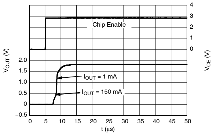
Figure 48. Start-up, 1.8 V Version, V_{IN} = 2.8 V
