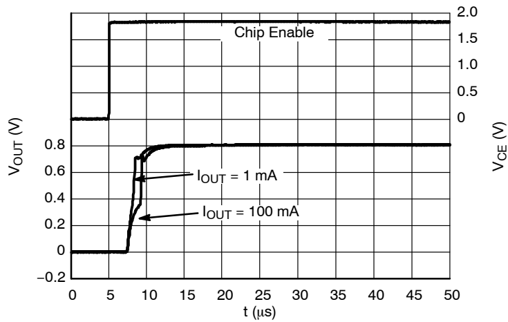
Figure 47. Start-up, 0.8 V Version, V_{IN} = 1.8 V
