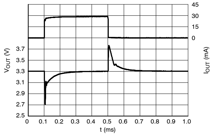
Figure 34. Load Transients, 3.3 V Version, I OUT = 1 – 30 mA, t R = t F = 0.5 μs, V IN = 4.3 V
