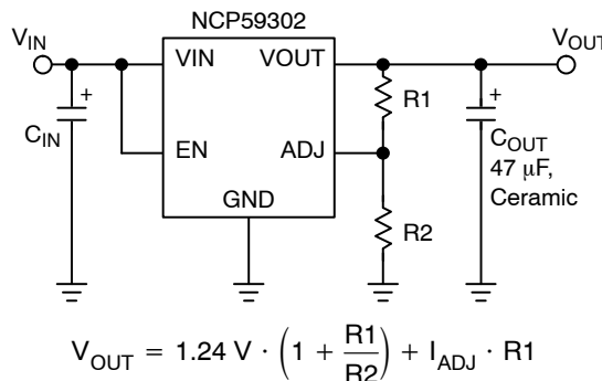
Figure 21. Adjustable Voltage Operation
