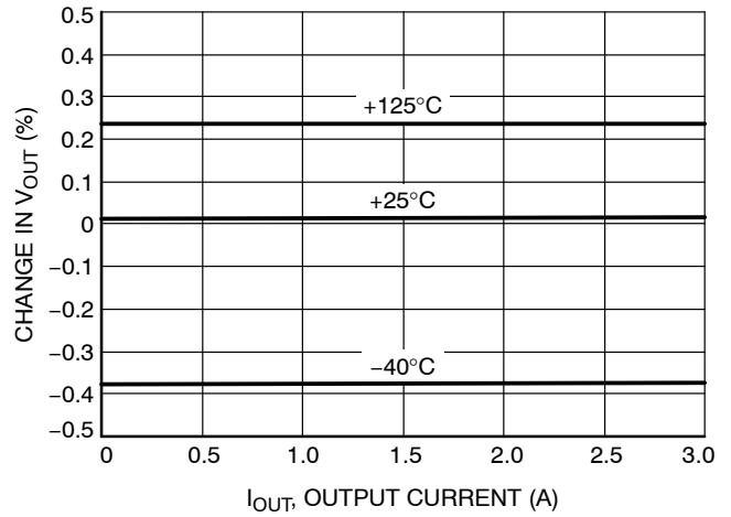
Figure 7. Load Regulation
