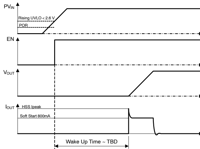
Figure 37. Power-Up Sequence
