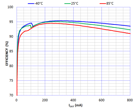
Figure 27. Efficiency vs Output Current vs Temperature PV_{IN} = 4.2\text{ V} , F_{sw} = 3.429\text{ MHz} , V_{OUT} = 3.3\text{ V}
