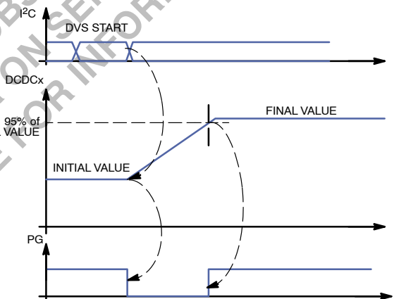
Figure 25. PG Operation in DVS Sequence
