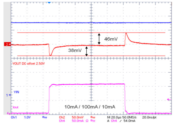
Figure 44. Load transient response LDO4, V_{OUT} = 2.50\text{ V}
