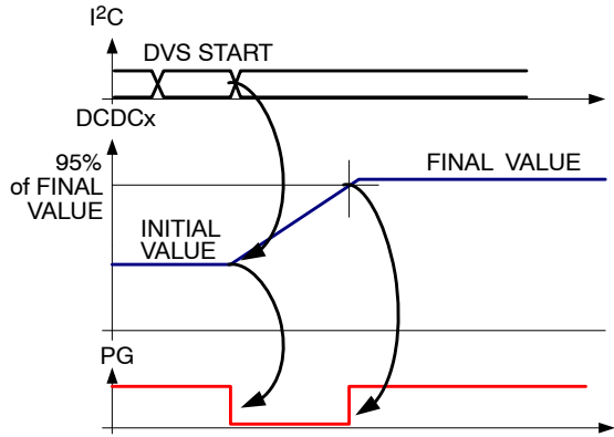
Figure 63. PG Operation in DVS Sequence
