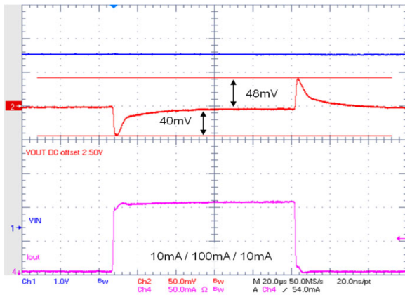
Figure 43. Load transient response LDO3, V_{OUT} = 2.50\text{ V}
