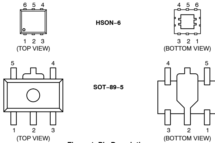
Figure 1. Pin Description
