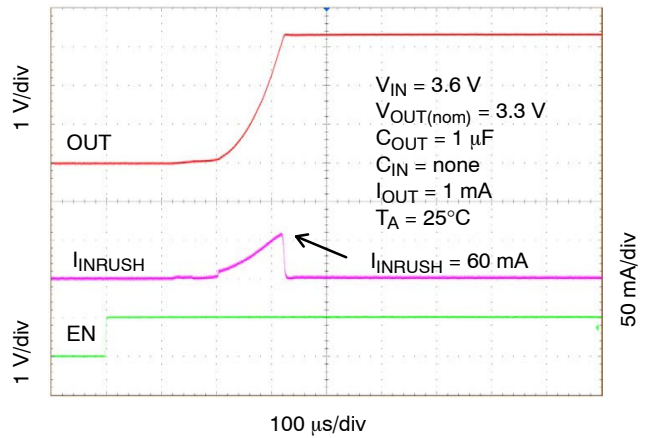
Figure 36. Enable Turn-On Response, V_{OUT} = 3.3\text{ V} , C_{OUT} = 1\ \mu\text{F}
