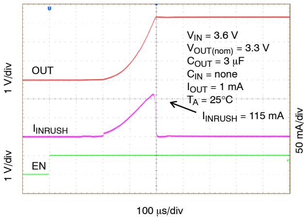
Figure 37. Enable Turn-On Response, V_{OUT} = 3.3\text{ V} , C_{OUT} = 3\ \mu\text{F}
