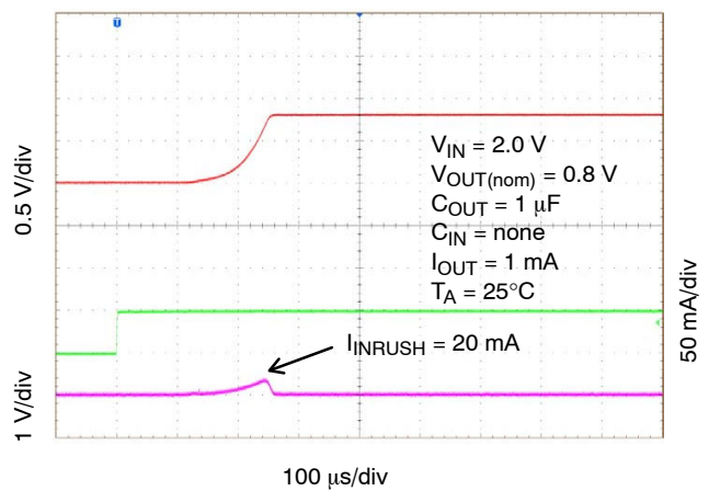
Figure 38. Enable Turn-On Response, V_{OUT} = 0.8\text{ V} , C_{OUT} = 1\ \mu\text{F}
