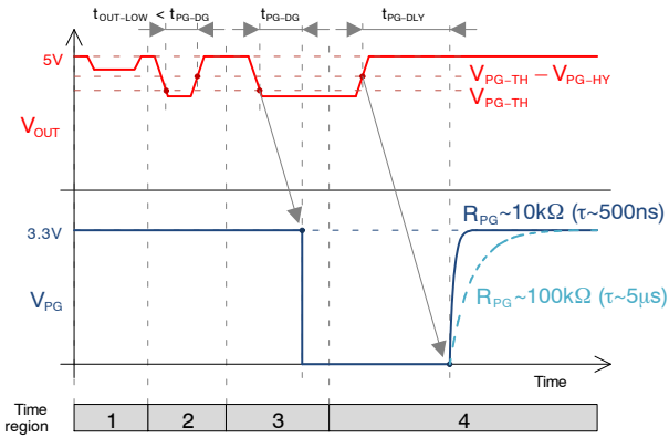
Figure 78. Timing – PG Connected to Application Power Supply 3.3 V
