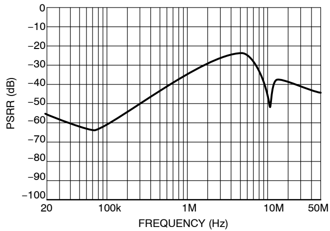
Figure 17. SD and HD V CC PSRR vs. Frequency
