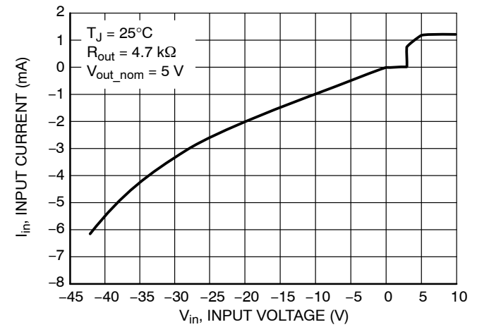
Figure 6. Input Current vs. Input Voltage (Reverse Input Voltage)
