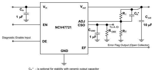
Figure 1. Application Schematic
