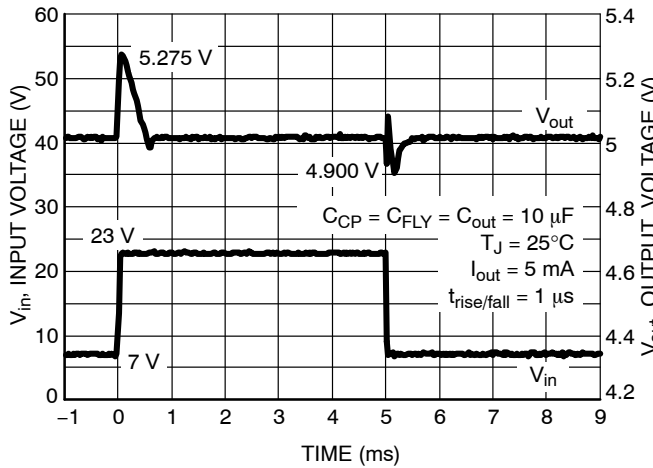
Figure 14. Line Transient
