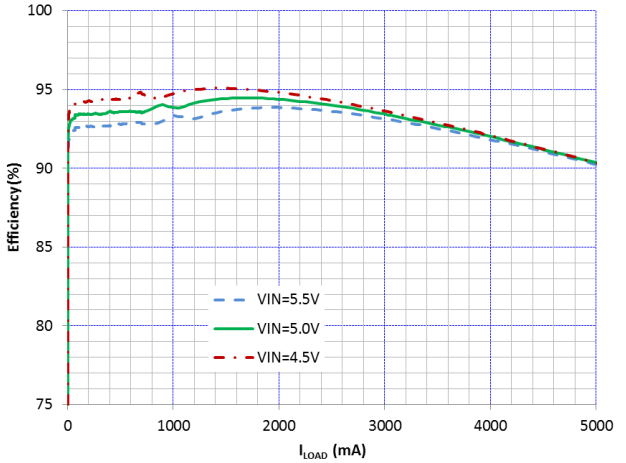
Figure 14. Efficiency vs I_{LOAD} and V_{IN} V_{OUT} = 3.30 V
