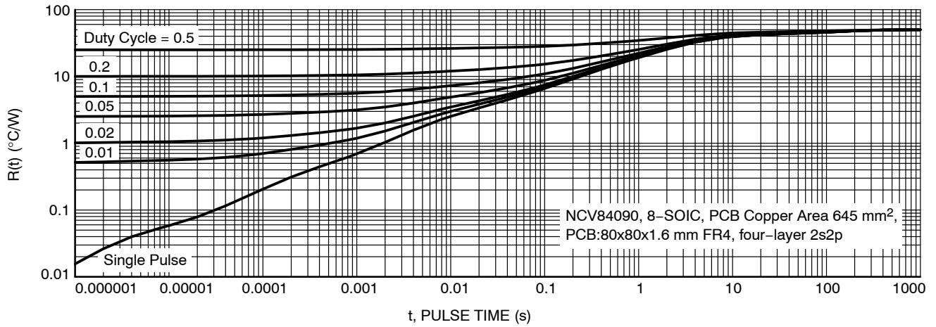
Figure 39. Junction-to-Ambient Transient Thermal Impedance ( 645 \text{ mm}^2 Cu Area)
