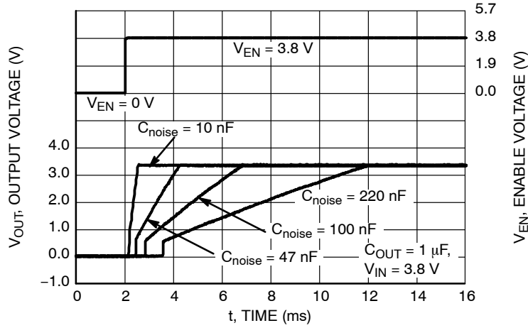
Figure 34. Turn-On Response V_{OUT} = 3.3 \text{ V} , C_{OUT} = 1 \mu\text{F} , I_{OUT} = 30 \text{ mA}
