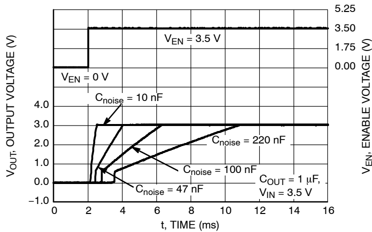
Figure 35. Turn-On Response V_{OUT} = 3 \text{ V} , C_{OUT} = 1 \mu\text{F} , I_{OUT} = 30 \text{ mA}
