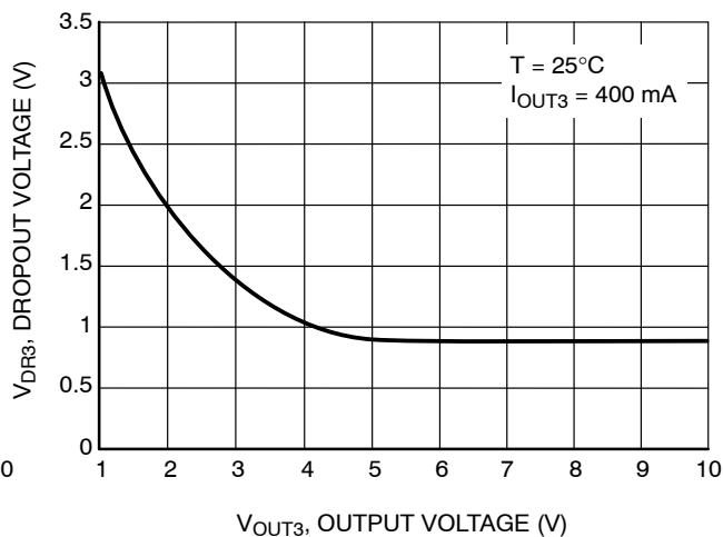
Figure 19. LDO3 Dropout Voltage vs. Output Voltage
