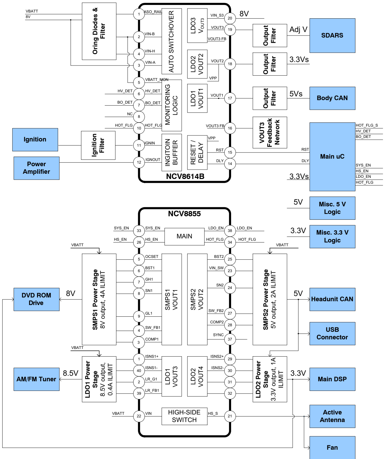
Figure 2. Automotive Radio System Block Diagram Example NCV8614B with NCV8855
