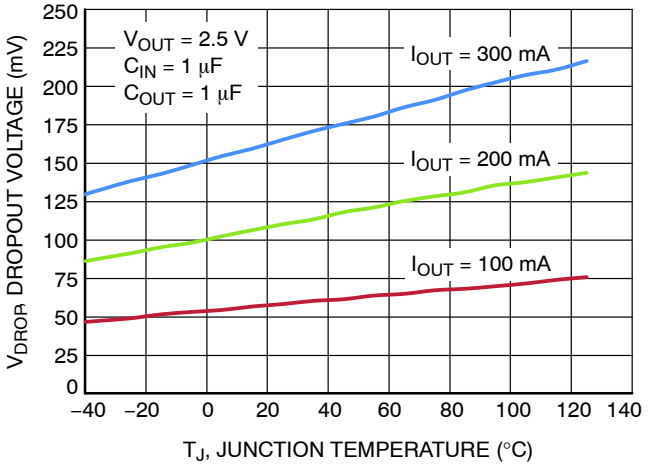
Figure 24. Dropout vs. Temperature – 2.5 V
