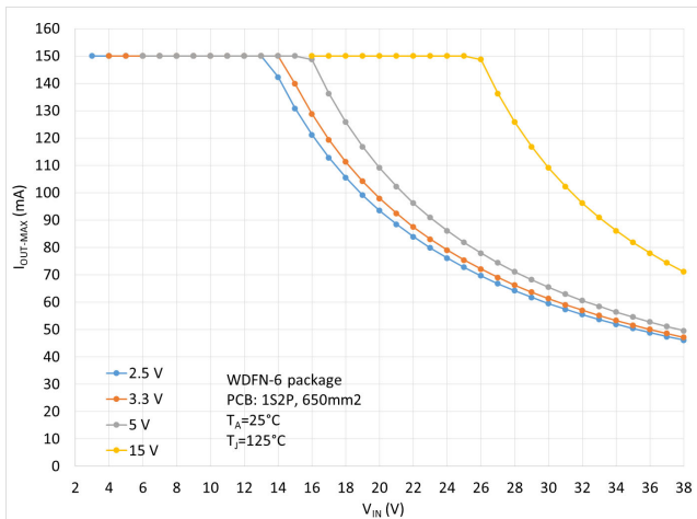
Figure 70. Maximum Output Current vs. Input Voltage
