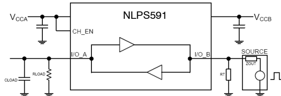
Figure 10. Rail-to-Rail Driving B-side I/O
