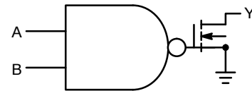
09 - AND with Open-Drain Output
