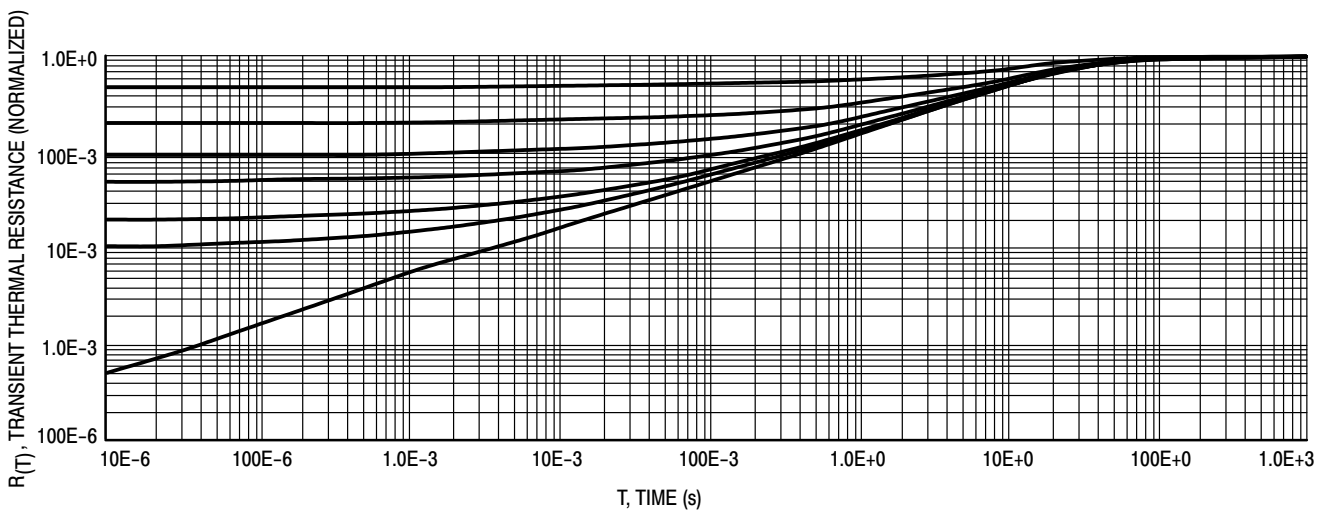
Figure 7. Thermal Response
