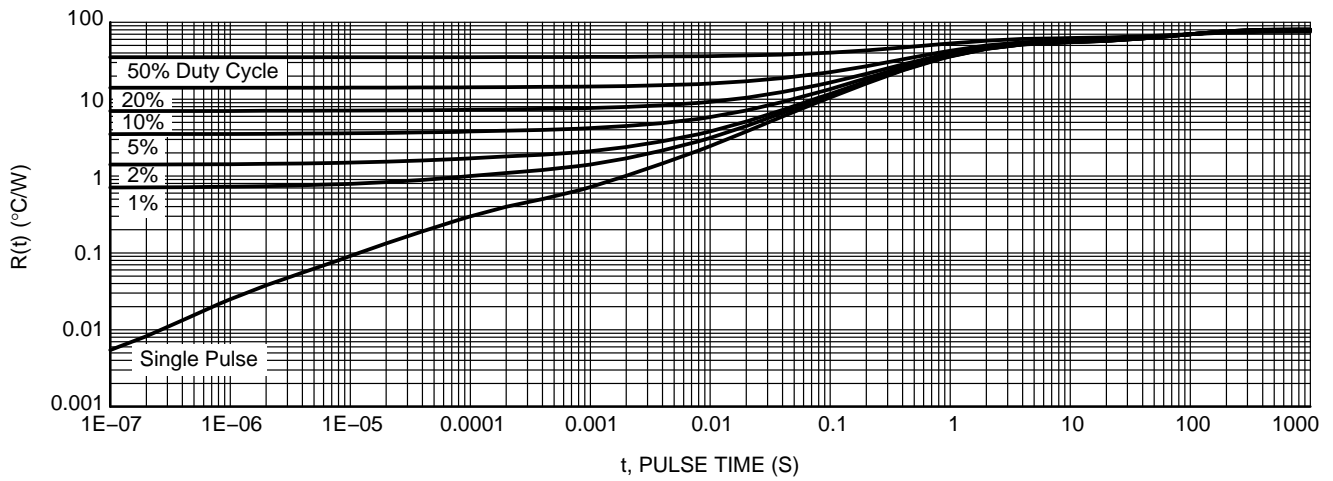
Figure 8. Typical Transient Thermal Response Characteristics, Junction-to-Ambient
