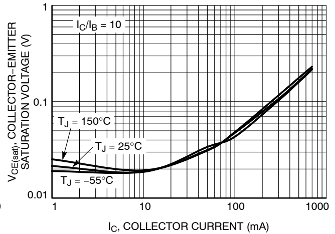
Figure 2. PNP V_{CE(sat)} vs. I_C
