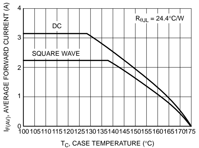
Figure 6. Current Derating
